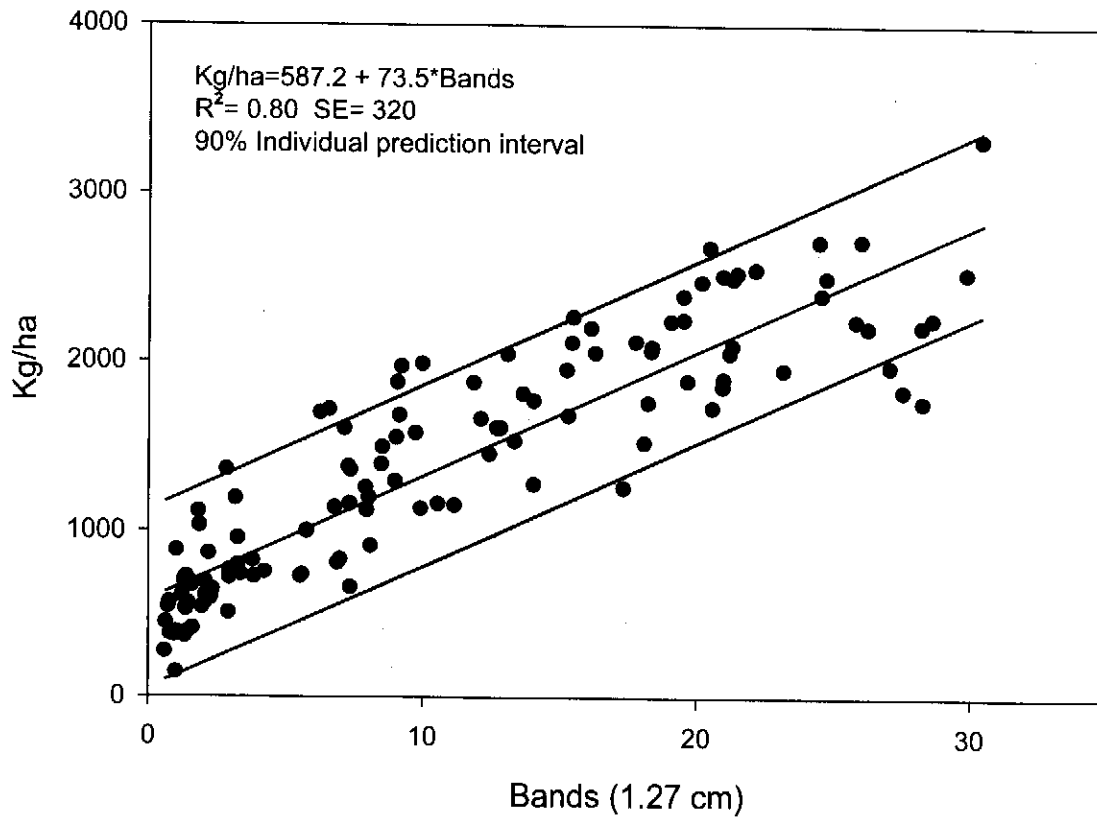
Figure 1. Regression relationship between Visual Obstruction Reading (VOR) bands and herbage ( \text{kg} \cdot \text{ha}^{-1} ) with 90% prediction bands for individual transects on the northern Black Hills, South Dakota, 2008.
